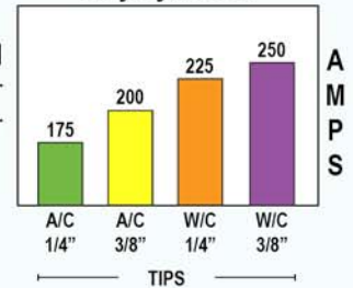
Duty Cycle 60%
